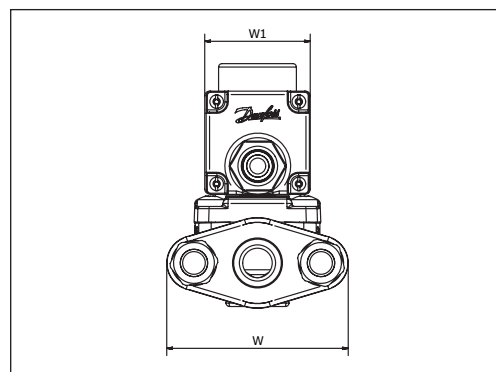
End view
